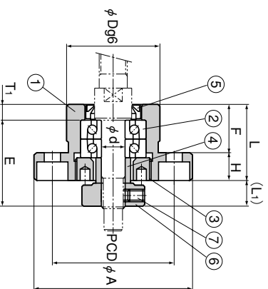
Mounting method A
