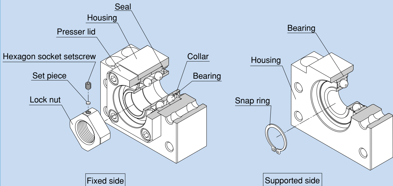
Fig. 1 Structure of the Support Unit
